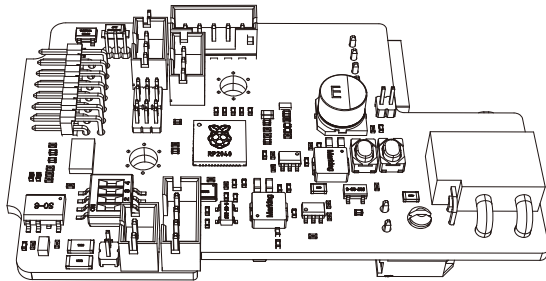
BIGTREETECH EBB SB2209 CAN V1.0 (RP2040)
